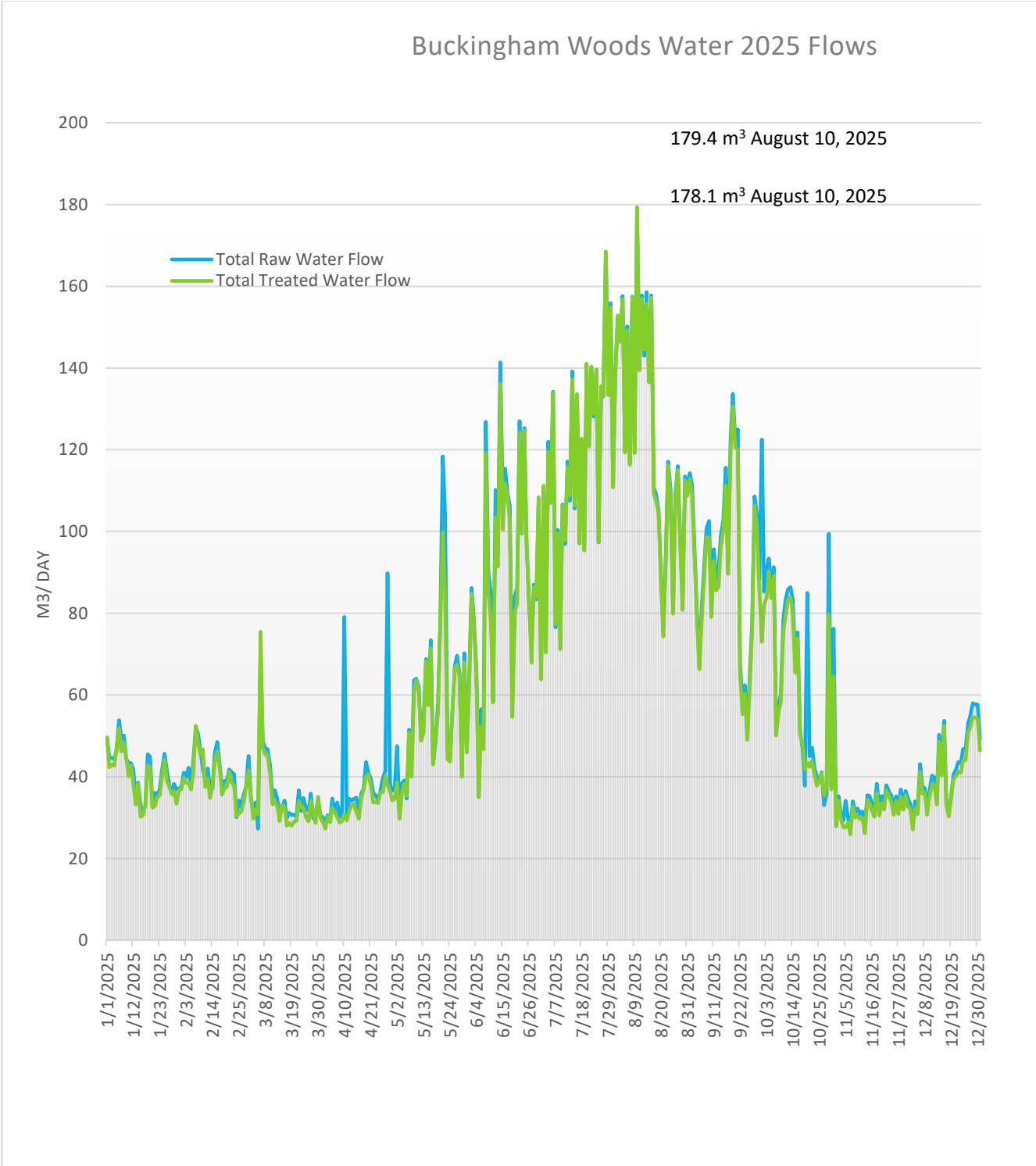
Figure 3: 2025 Daily Flows
