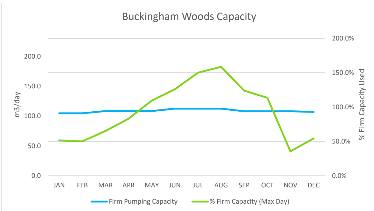
Figure 2: System Capacity
