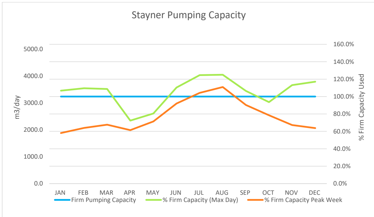
Figure 2: System Capacity
